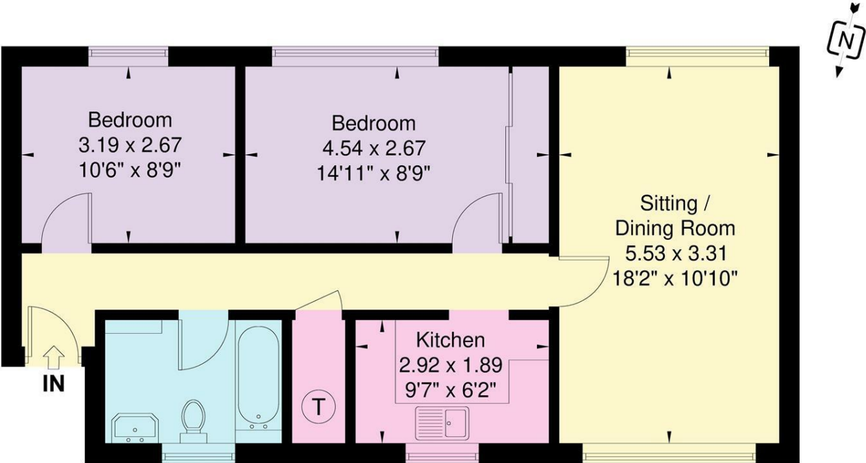
Second Floor
